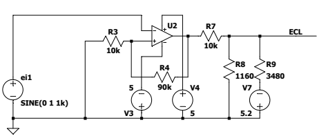
Regenerative comparator with the ECL logic gate
