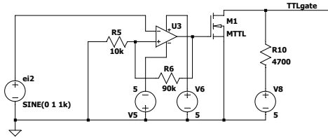
Regenerative comparator with TTL logic gates
